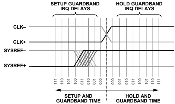
Figure 101. SYSREF± Edge Changes Phase Relative to the Encode Clock, Which can be Detected When the Edge Crosses Through the Guardband Setup Time
