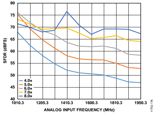
Figure 130. Buffer Current Sweeps, AD9680-500 (SFDR vs. I_{BUFF} ); 1 GHz < f_{IN} < 2 GHz; Front-End Network Shown in Figure 115
