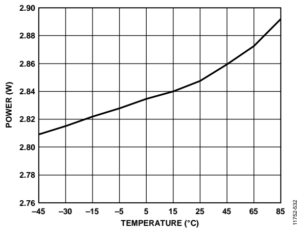
Figure 78. Power Dissipation vs. Temperature
