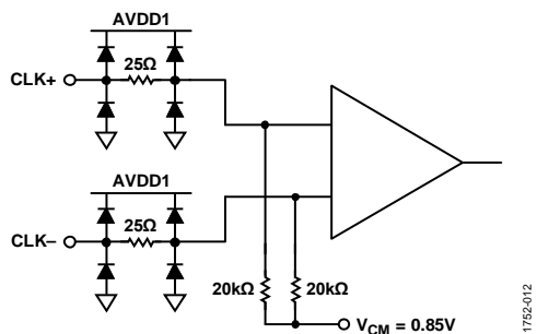
Figure 105. Clock Inputs
