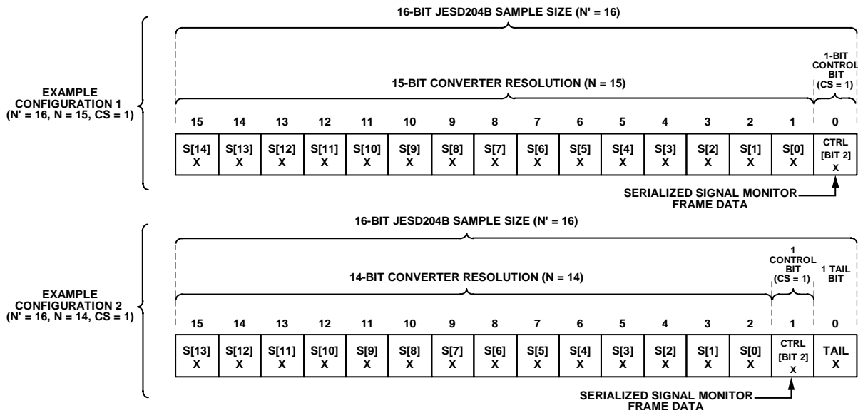
Figure 143. Signal Monitor Control Bit Locations
