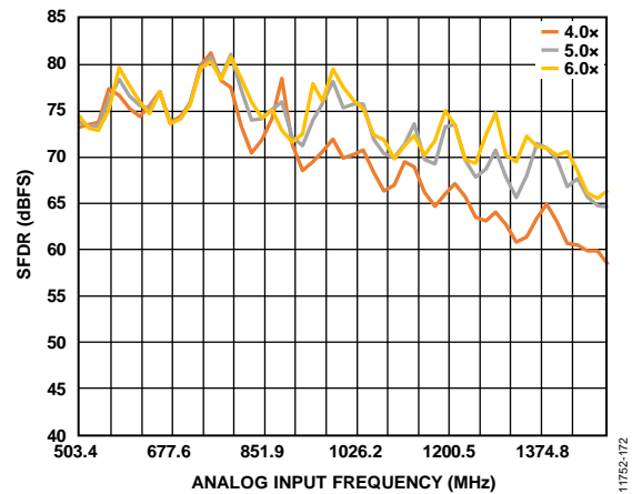
Figure 122. Buffer Current Sweeps, AD9680-1000 (SFDR vs. I_{BUFF} ); 500 \text{ MHz} < f_{IN} < 1500 MHz; Front-End Network Shown in Figure 115
