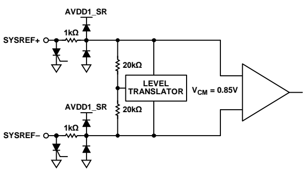
Figure 106. SYSREF± Inputs
