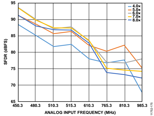
Figure 129. Buffer Current Sweeps, AD9680-500 (SFDR vs. I_{BUFF} ); 450 MHz < f_{IN} < 1000 MHz; Front-End Network Shown in Figure 115
