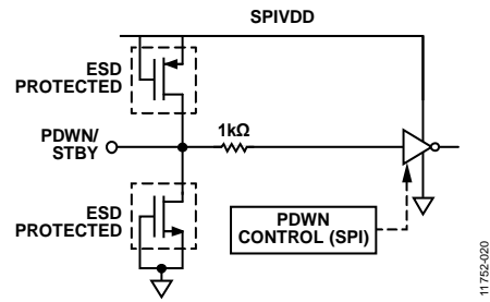
Figure 113. PDWN/STBY Input
