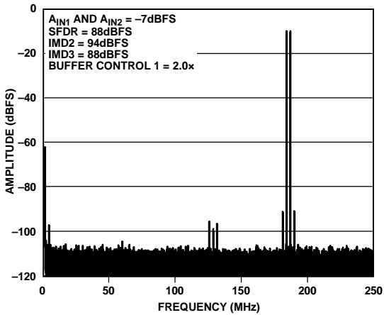
Figure 93. Two-Tone FFT; f_{IN1} = 184\text{ MHz} , f_{IN2} = 187\text{ MHz}
