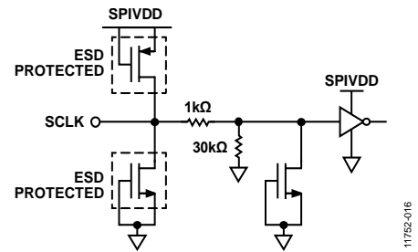
Figure 109. SCLK Input
