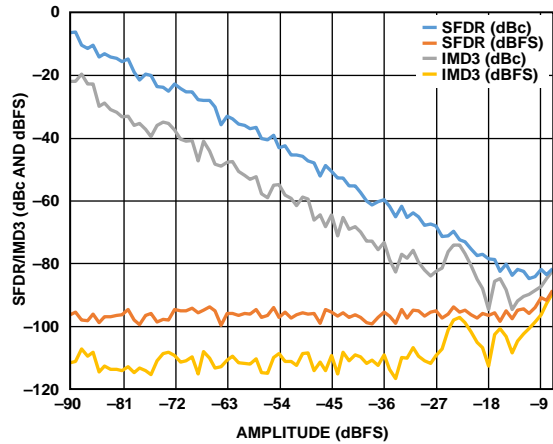
Figure 96. Two-Tone IMD3/SFDR vs. Input Amplitude ( A_{IN} ) with f_{IN1} = 338\text{ MHz} and f_{IN2} = 341\text{ MHz}
