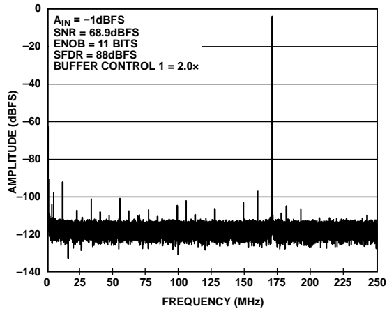
Figure 81. Single-Tone FFT with f_{IN} = 170.3 MHz
