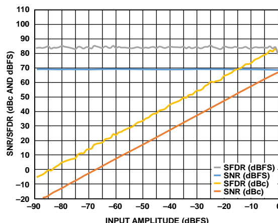
Figure 97. SNR/SFDR vs. Analog Input Level, f_{IN} = 170.3\text{ MHz}
