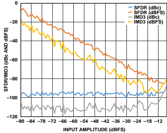
Figure 95. Two-Tone SFDR/IMD3 vs. Input Amplitude ( A_{IN} ) with f_{IN1} = 184\text{ MHz} and f_{IN2} = 187\text{ MHz}
