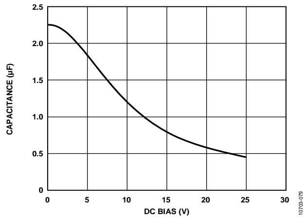
Figure 81. Capacitance vs. DC Bias Characteristics
