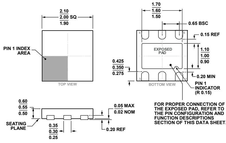
Figure 104. 6-Lead Lead Frame Chip Scale Package [LF CSP] 2.00 mm × 2.00 mm Body and 0.55 Package Height (CP-6-3) Dimensions shown in millimeters
