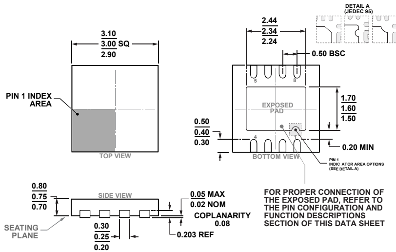
COMPLIANT TO JEDEC STANDARDS MO-229-W3030D-4 Figure 105. 8-Lead Lead Frame Chip Scale Package [LF CSP] 3 mm × 3 mm Body and 0.75 Package Height (CP-8-11) Dimensions shown in millimeters
