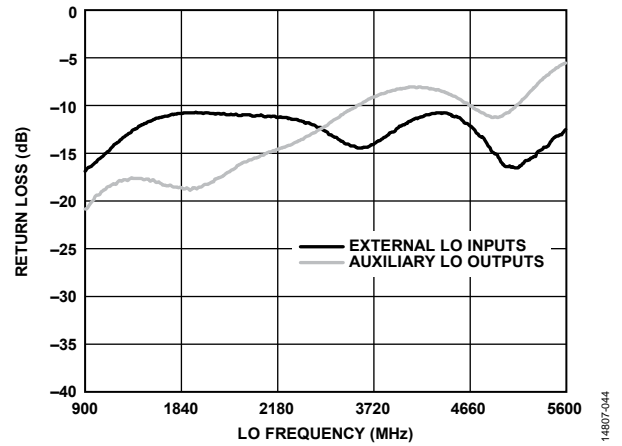
Figure 44. Return Loss vs. LO Frequency for Auxiliary LO Outputs and External LO Inputs
