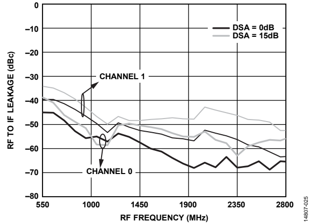
Figure 25. RF to IF Leakage at IF Output
