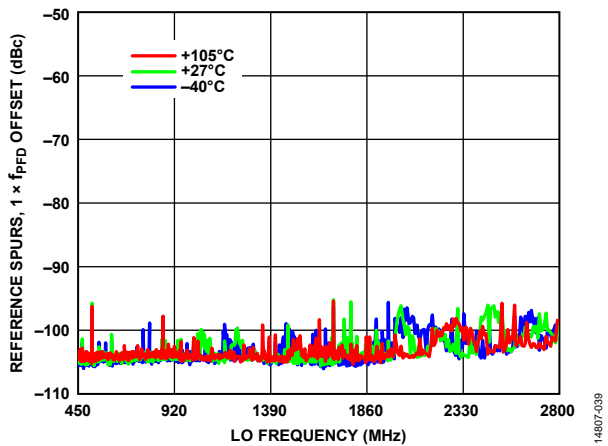
Figure 39. Reference Spurs, 1 \times f_{PFD} Offset vs. LO Frequency
