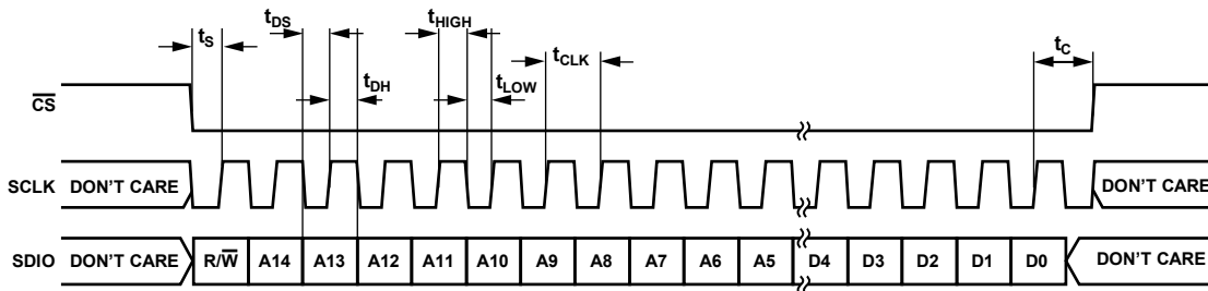
Figure 2. SPI Write (MSB First), 16-Bit Instruction, Timing Measurements
