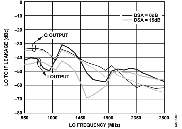
Figure 26. LO to IF Leakage at IF Output
