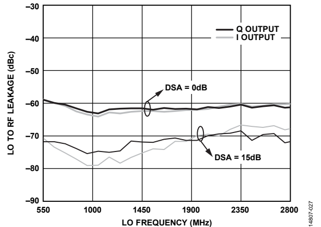
Figure 27. LO to RF Leakage vs. LO Frequency
