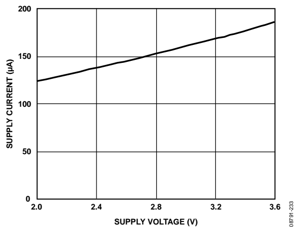
Figure 20. Supply Current vs. Supply Voltage, V_S at 25^\circ\text{C}
