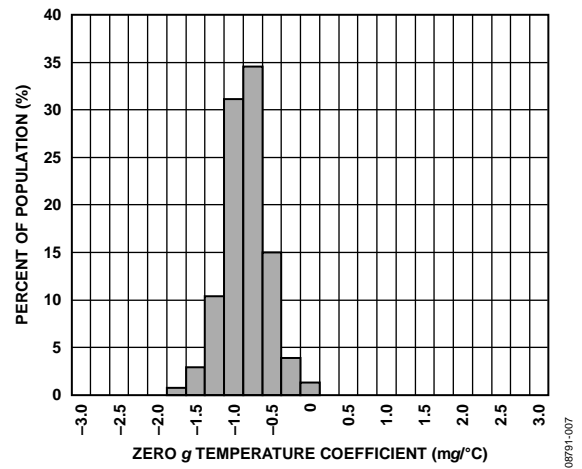
Figure 7. Y-Axis Zero-g Bias Drift, V_S = V_{DD/IO} = 3.3 V
