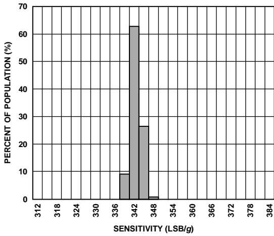
Figure 9. X-Axis Sensitivity, V_S = V_{DD/IO} = 3.3\text{ V} , 25^\circ\text{C}
