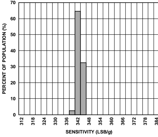
Figure 10. Y-Axis Sensitivity, V_S = V_{DD/IO} = 3.3\text{ V} , 25^\circ\text{C}
