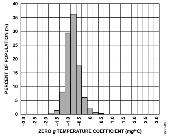
Figure 6. X-Axis Zero-g Bias Drift, V_S = V_{DD/IO} = 3.3 V
