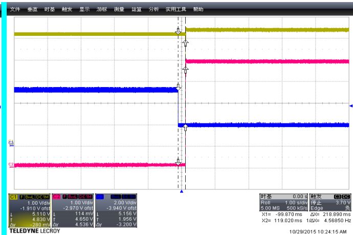
Fig:23 At 265Vac_Rising time = 218mS at 3A load
