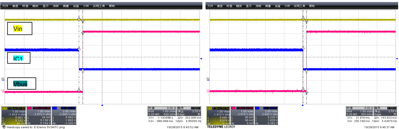
Fig:22 At 90Vac_Rising time =202mS at 0A load
