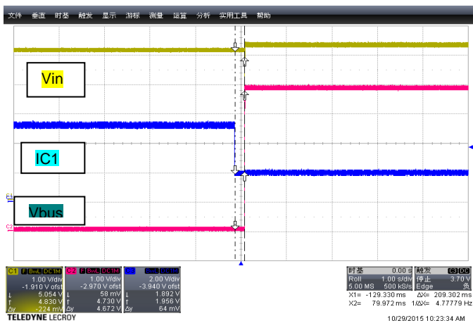
Fig:22 At 90Vac_Rising time =209mS at 3A load
