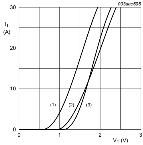
V_o = 1.264\text{ V} R_s = 0.038\ \Omega (1) T_j = 125^\circ\text{C} ; typical values (2) T_j = 125^\circ\text{C} ; maximum values (3) T_j = 25^\circ\text{C} ; maximum values Fig. 10. On-state current as a function of on-state voltage
