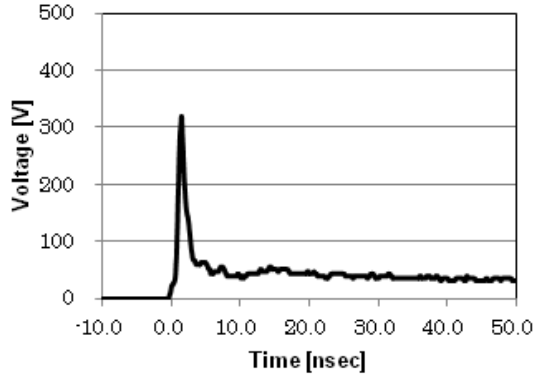
ESD Waveform (IEC61000-4-2:8kV Contact)
