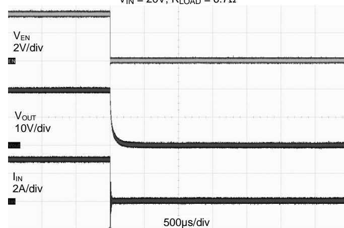
EN Turn OFF with a 7\Omega Load at 20V
