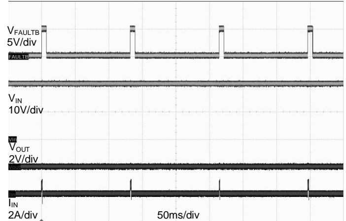
Overcurrent Recovery at 5V
