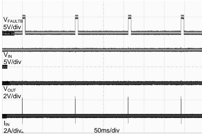
Overcurrent Protection at 5V
