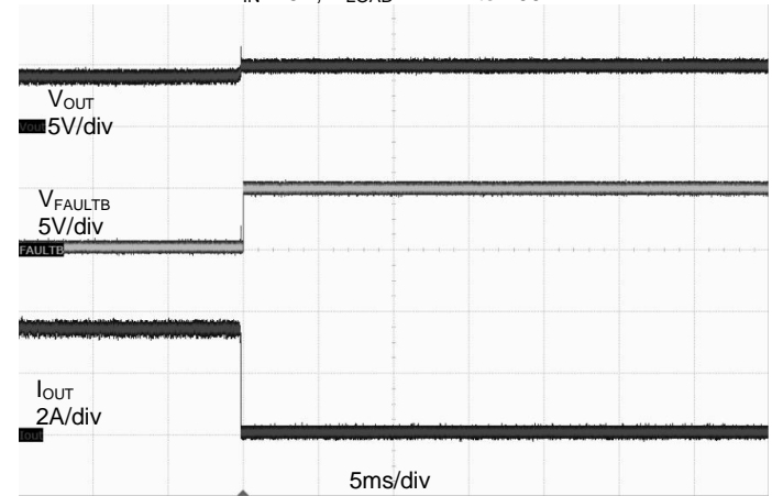
Reverse-voltage Response
