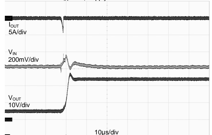
Reverse-voltage Response
