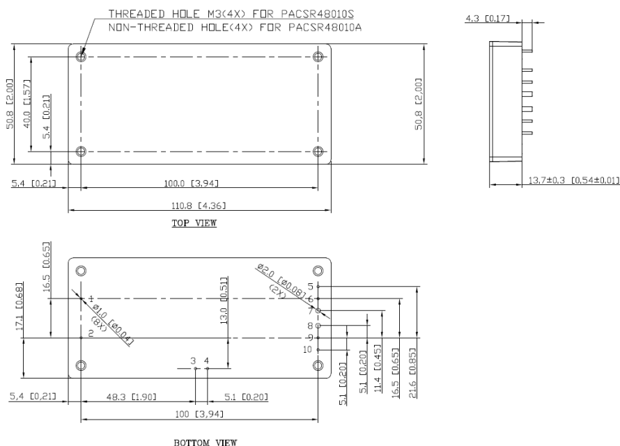
Mechanical Dimensions
