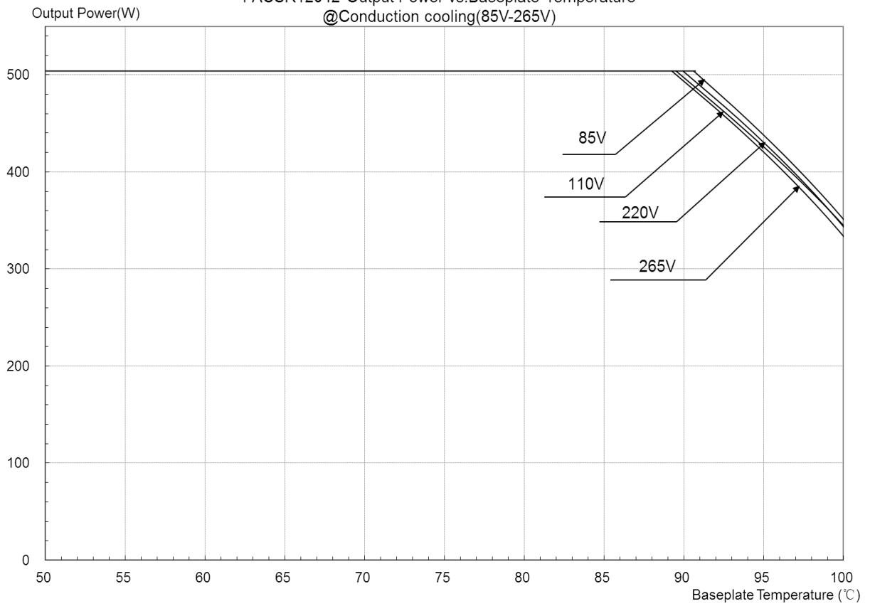
Figure 12: Thermal derating curves
