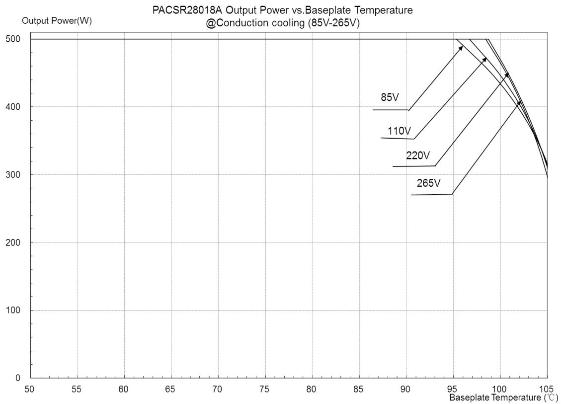
Figure 12: Thermal derating curve
