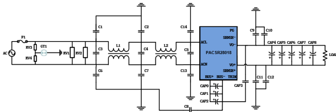
Figure 9: Application connection
