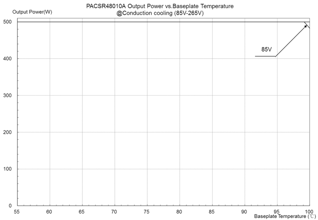
Figure 12: Thermal derating curves
