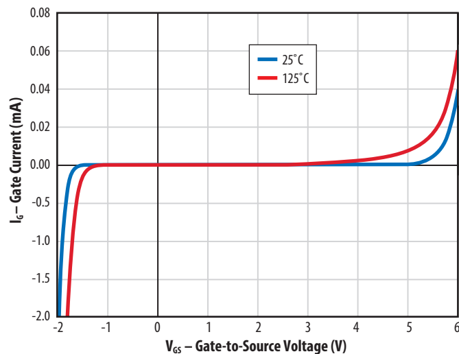
Figure 13 (Q3): Gate-Source Characteristics
