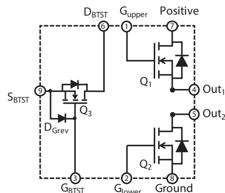
EPC2107 – Detailed Schematic
