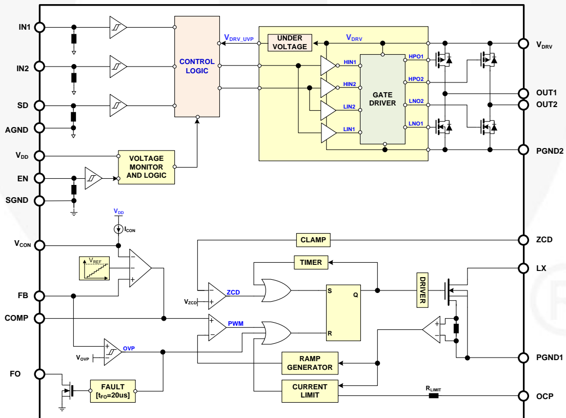
Figure 2. Block Diagram
