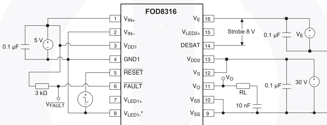
Figure 43. DESAT Sense ( t_{DESAT(90\%)} , t_{DESAT(10\%)} ), DESAT Fault ( t_{DESAT(FAULT)} ), and ( t_{DESAT(LOW)} ) Test Circuit
