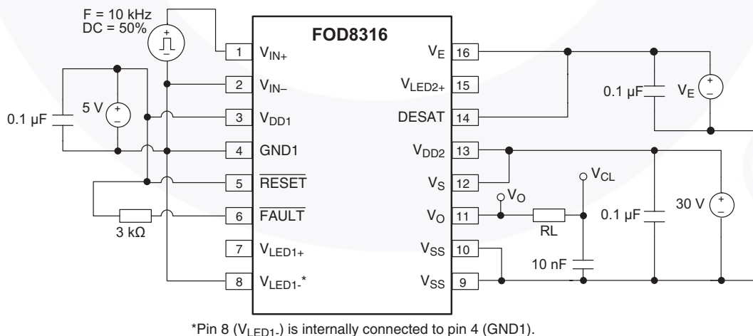
Figure 42. Propagation Delay ( t_{PLH} , t_{PHL} ), Pulse Width Distortion (PWD), Rise Time ( t_R ) and Fall Time ( t_F ) Test Circuit
