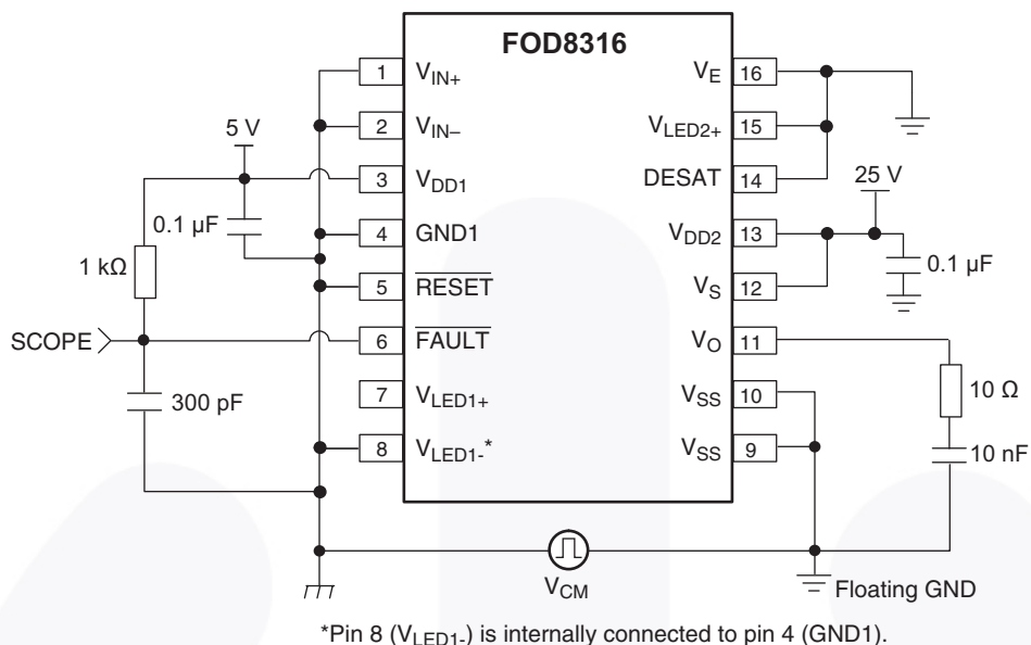
Figure 48. Common Mode High ( CM_H ) Test Circuit @ LED2 Off
