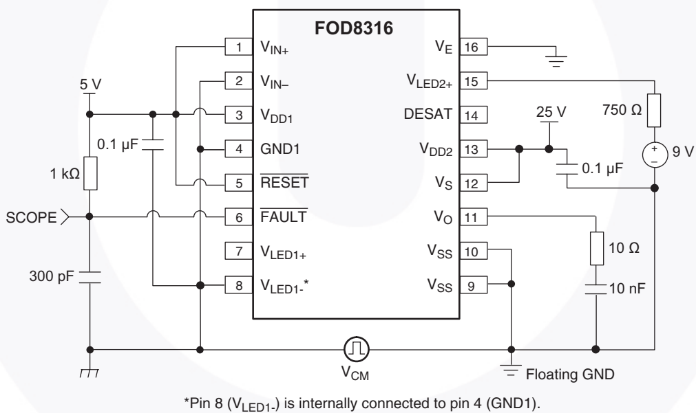
Figure 49. Common Mode Low ( CM_L ) Test Circuit @ LED2 On
