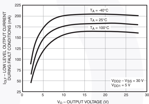
Figure 6. Low Level Output Current ( I_{\text{OLF}} ) vs. Output Voltage ( V_O )
