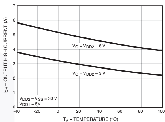
Figure 4. Output High Current ( I_{\text{OH}} ) vs. Temperature
