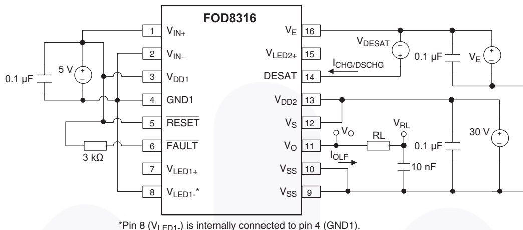
Figure 40. Low Level Output Current During Fault Conditions ( I_{OLF} ), Blanking Capacitor Charge Current ( I_{CHG} ), Blanking Capacitor Discharging Current ( I_{DSCHG} ) and DESAT Threshold ( V_{DESAT} ) Test Circuit
