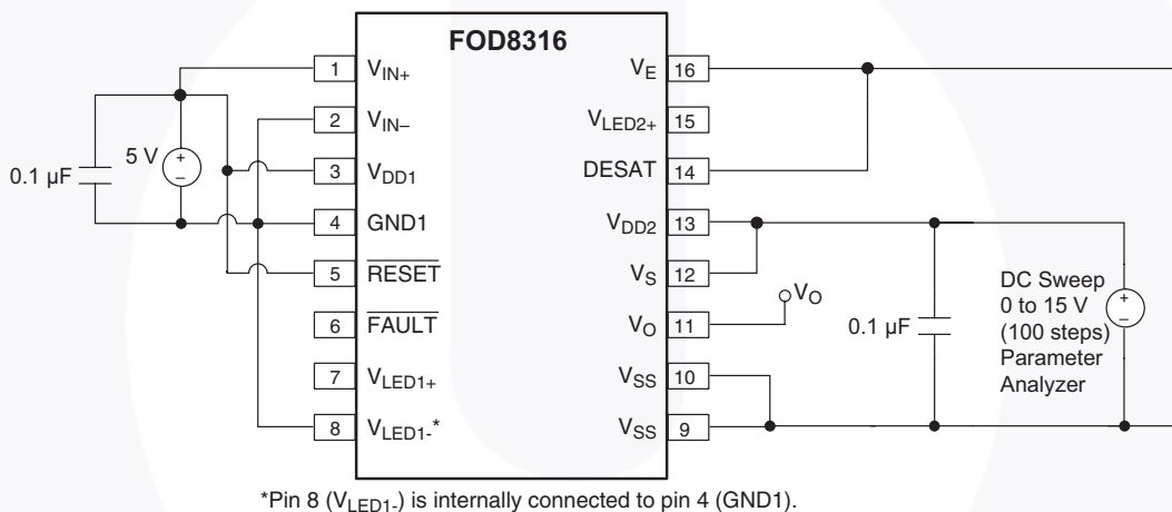
Figure 41. Under Voltage Lockout Threshold ( V_{UVLO} ) Test Circuit
