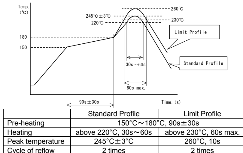
Reflow soldering profile
