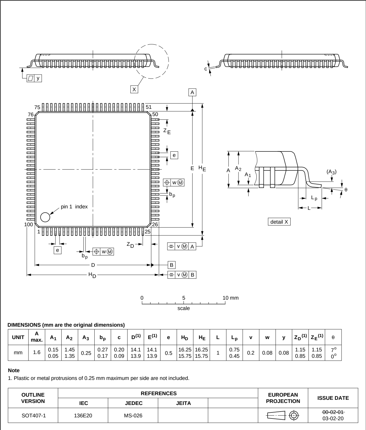
Fig 50. LQFP100 package
