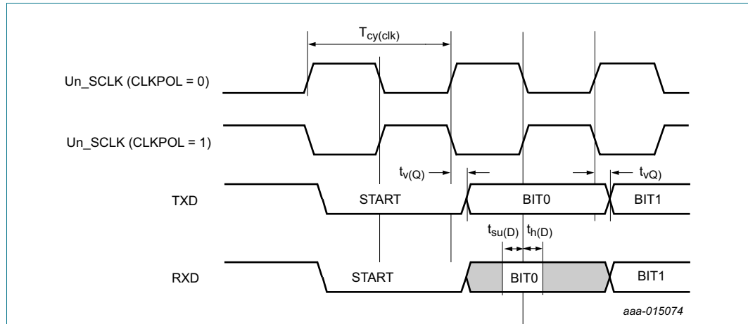
Fig 34. USART timing
