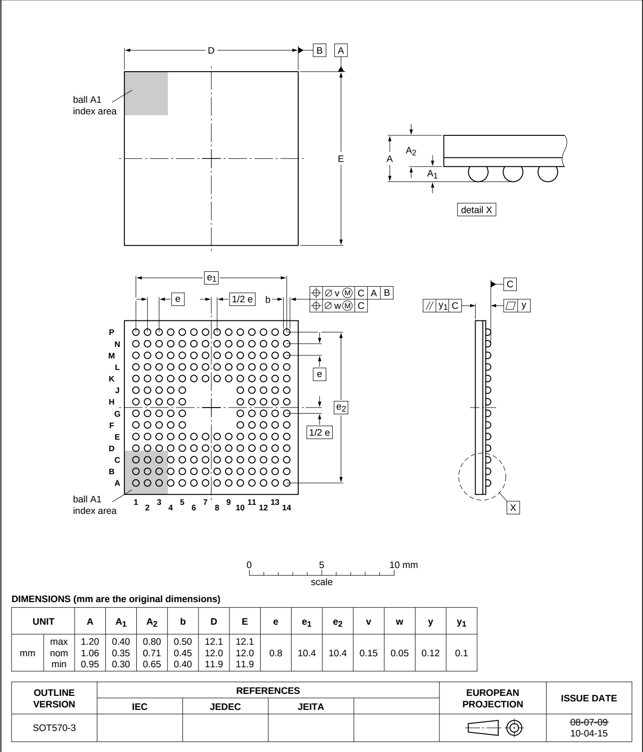
Fig 51. TFBGA180 package
