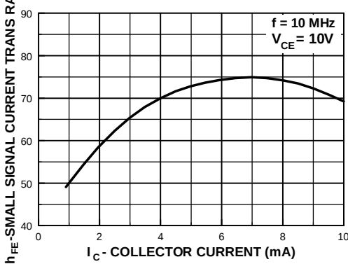
Small Signal Current Gain vs Collector Current
