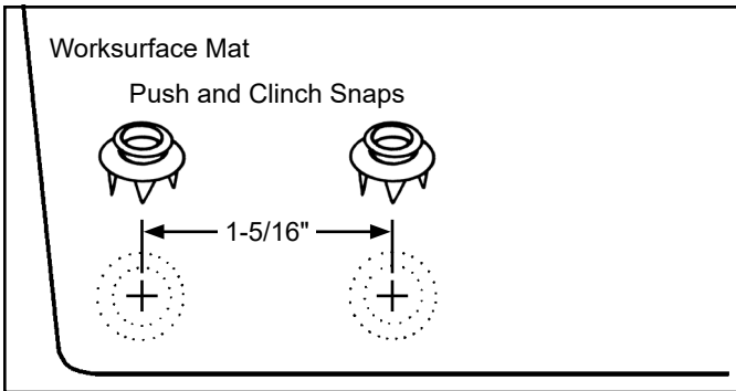
Figure 5. Installing the push and clinch snaps to the front edge of a worksurface mat
