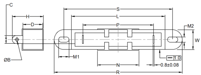
Figure 2 - soldered tag with rugged bracket (SR)
