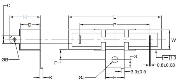
Figure 1 - soldered tag (S) and the same with bracket (SB)
