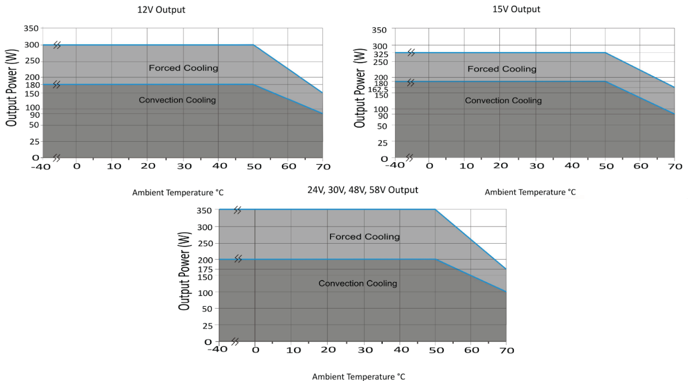
Figure 1 – Derating Curves
