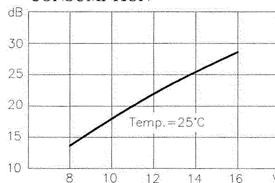
VOLTAGE-CURRENT CONSUMPTION
