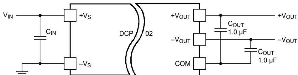
Figure 10. Dual Output Devices Connected in Series
