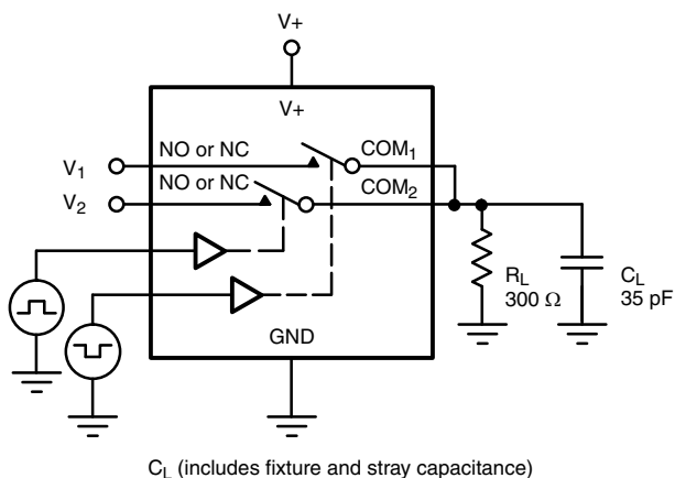
Fig. 2 - Break-Before-Make Interval
