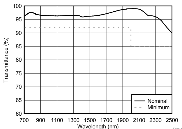
Figure 6. DLP4500NIR DMD Window Transmittance
