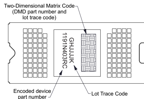
Figure 19. Device Marking for FQD
