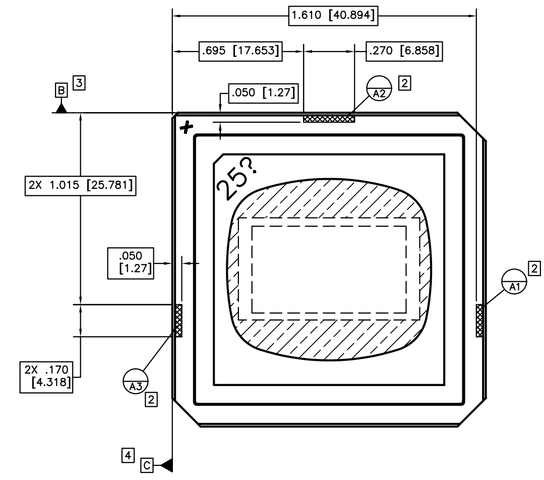
VIEW A (SHEET 1 NOTES) DATUM A, B AND C DETAILS
