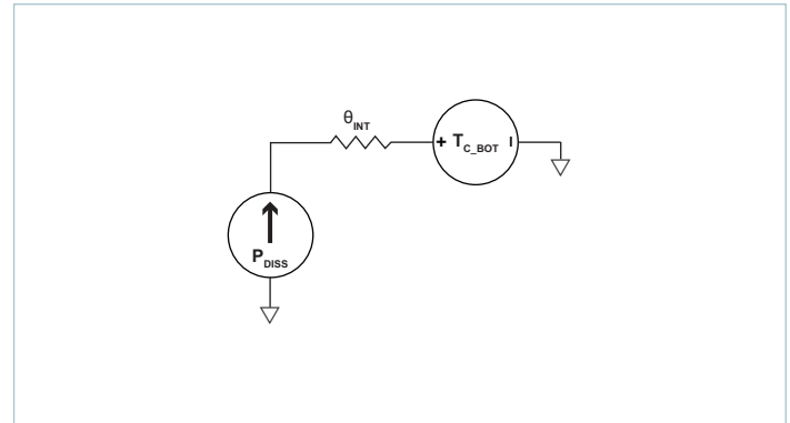
Figure 23 — Single-sided cooling VIA thermal model
