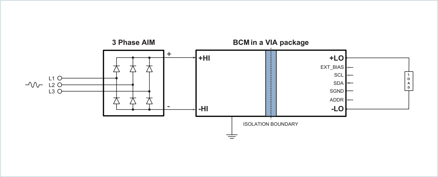
3 phase AC to point of load (3 phase AIM + BCM4414xG0F4440yzz)
