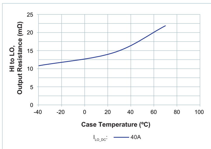
Figure 12 — R_{LO} vs. temperature; Nominal V_{HI\_DC} I_{LO\_DC} = 40\text{A} at T_{CASE} = 70^{\circ}\text{C}
