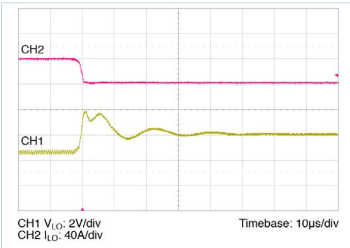
Figure 16 — 40A – 0A transient response: no external C_{HI\_IN\_EXT} ; no external C_{LO\_OUT\_EXT}
