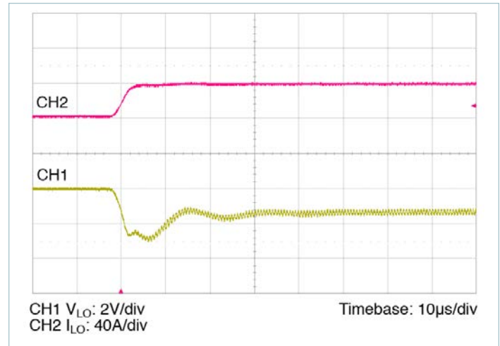
Figure 15 — 0A – 40A transient response: no external C_{HI\_IN\_EXT} ; no external C_{LO\_OUT\_EXT}
