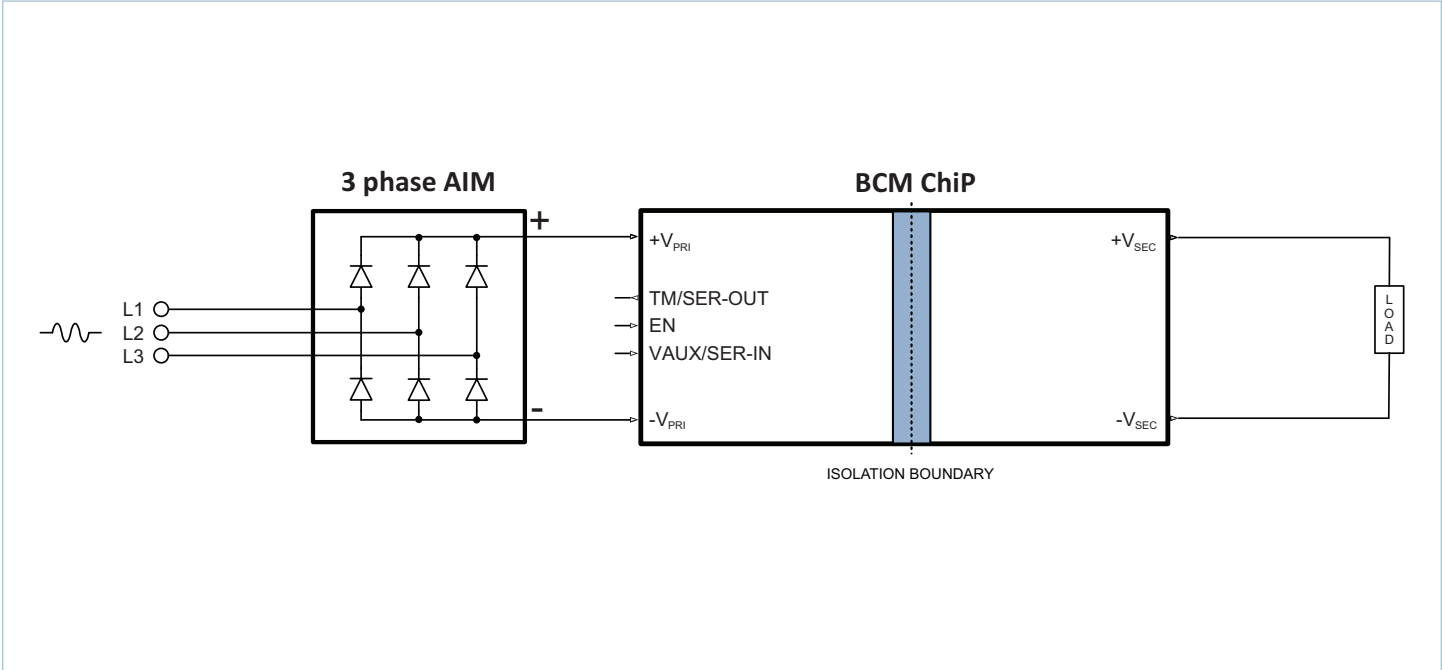
3 phase AC to point of load (3 phase AIM + BCM6123xD1E1368yzz)
