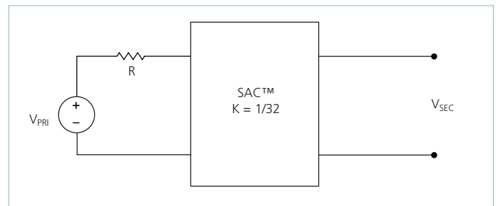
Figure 20 — K = 1/32 Sine Amplitude Converter with series primary resistor
