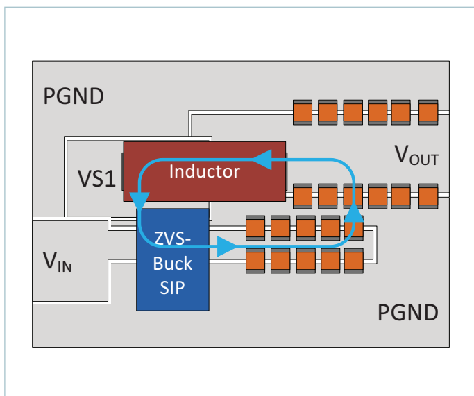
Figure 94 — Recommended layout for Optimized AC Current within the SiP, Inductor, and Ceramic Input and Output Capacitors
