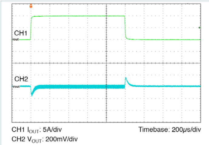
Figure 46 — Transient Response: 50% to 100% load, at 1A/µs. Nominal Line, Nominal Trim, C OUT = 12 x 47µF Ceramic
