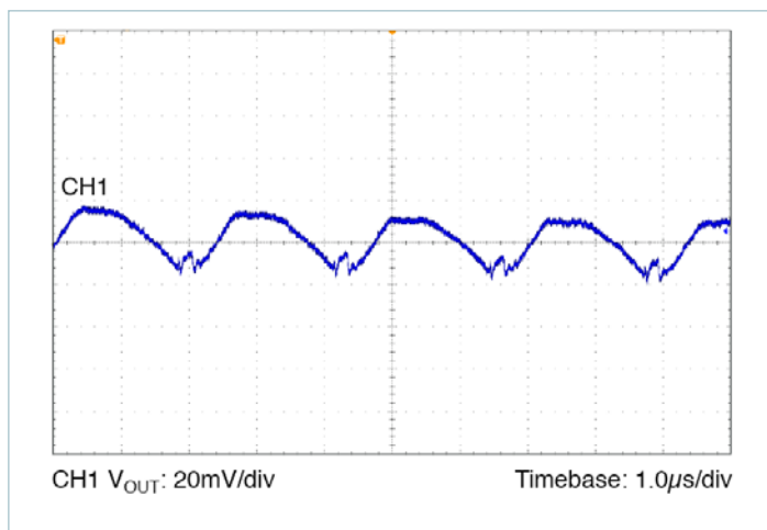
Figure 23 — Output Voltage Ripple: Nominal Line, Nominal Trim, 50% load, C OUT = 8 x 100μF Ceramic
