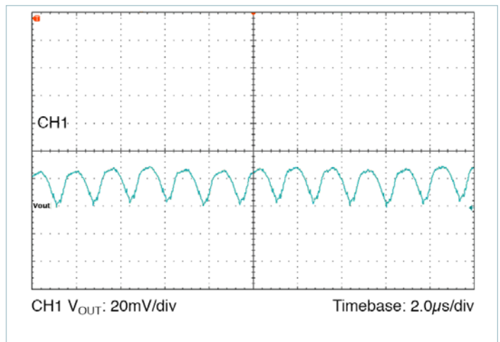
Figure 50 — Output Voltage Ripple: Nominal Line, Nominal Trim, 50% load, C OUT = 12 x 47µF Ceramic
