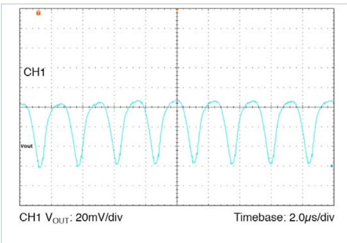
Figure 47 — Output Voltage Ripple: Nominal Line, Nominal Trim, 100% load, C OUT = 12 x 47µF Ceramic
