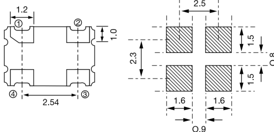
Figure 2) Land Pattern
