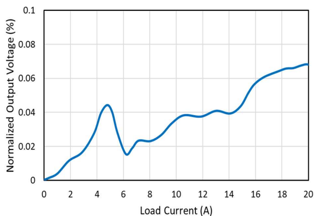
EM2120L Load Regulation, V_{OUT} = 0.9V
