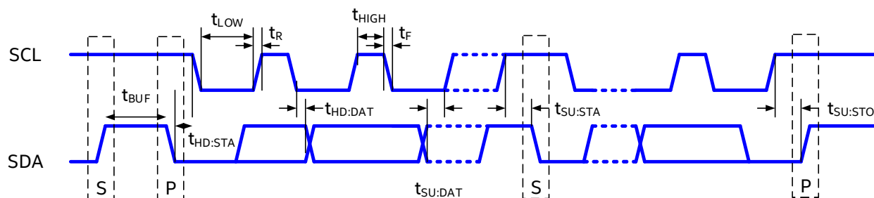
Figure 14: PMBus Timing Diagram
