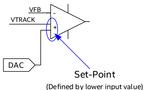
Figure 9: VTRACK Circuitry
