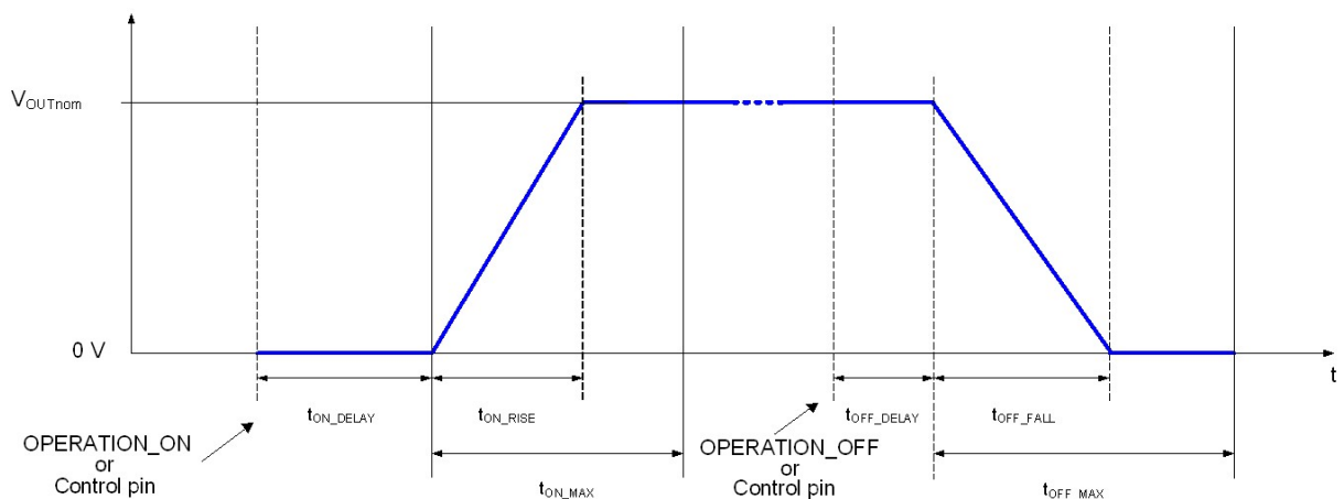
Figure 6: Power Sequencing
