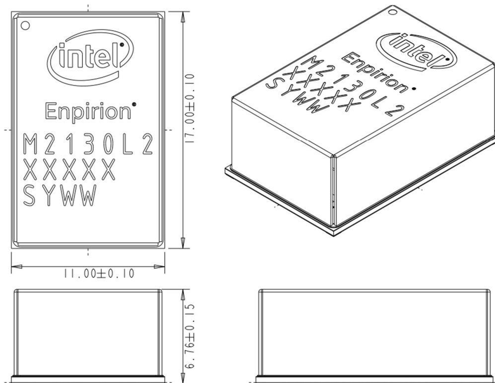
Figure 22: Package Dimensions (EM2130L02 Shown)
