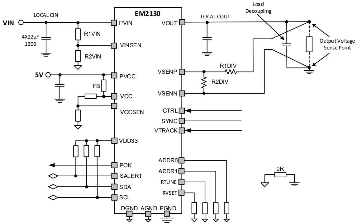
Figure 15: Recommended Application Circuit
