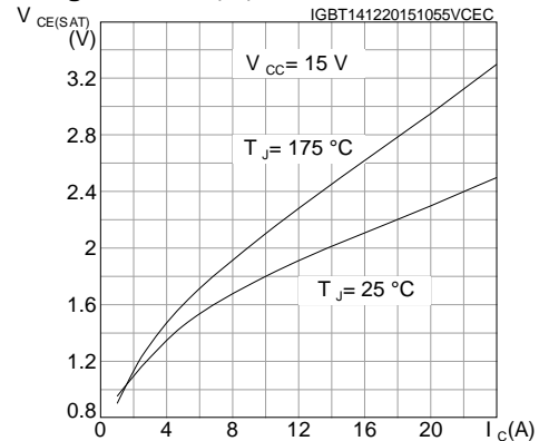
Figure 11: V_{CE(sat)} vs collector current
