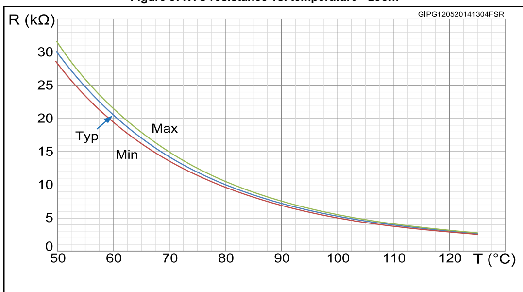
Figure 9: NTC resistance vs. temperature - zoom
