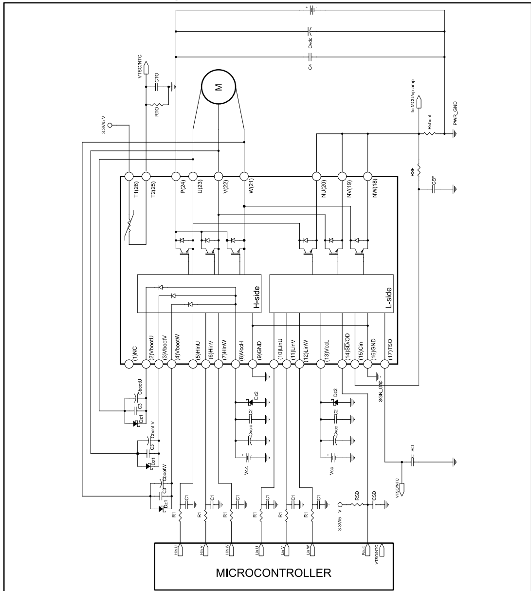
Figure 7: Application circuit example
