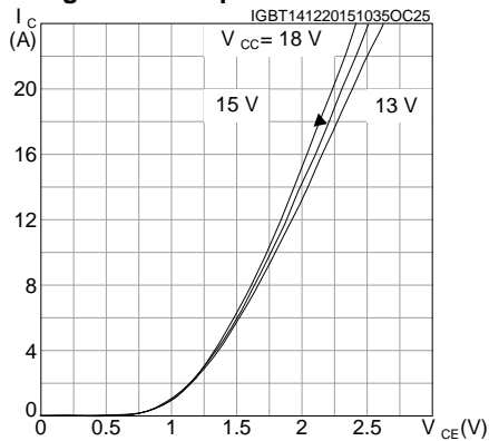
Figure 10: Output characteristics
