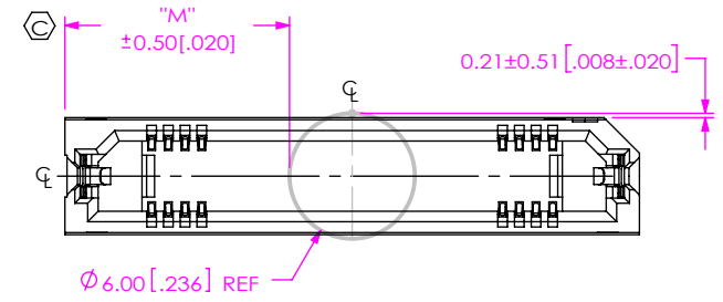
FIG 5 (ERF8-025-05.0-X-DV-L-K SHOWN) (SAME AS FIG 1 & 2, EXCEPT AS SHOWN) (AVAILABLE ON -05.0 & -07.0 LEAD STYLE ONLY) (CENTER FEATURES REMOVED FOR CLARITY)
