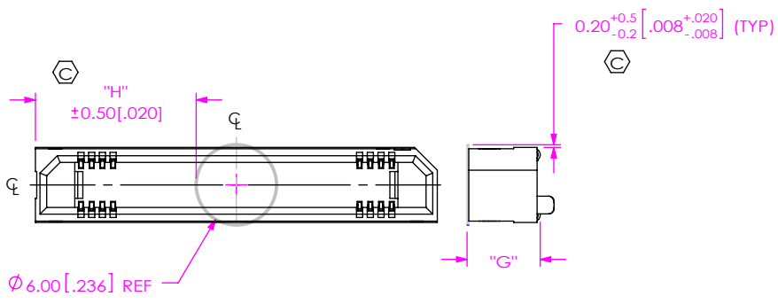
FIG 2 -K OPTION (USE K-DOT-.236-.343-.005) (ERF8-030-XX.X-X-DV-K SHOWN)
