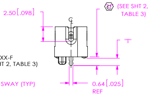
DETAIL "G" SCALE 6 : 1
