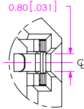
DETAIL "E" SCALE 6 : 1
