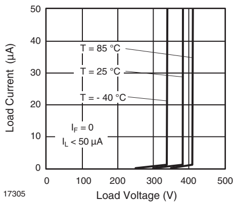
Fig. 6 - Switch Breakdown Voltage vs. Load Current
