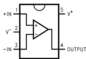
DBV and DCK Package 5-Pin SC70, SOT-23 Top View
