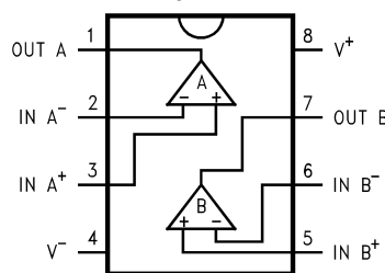
D and DGK Package 8-Pin SOIC, VSSOP Top View
