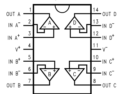
D and PW Package 14-Pin SOIC, TSSOP Top View
