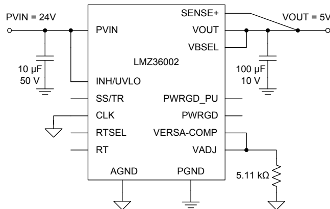
Figure 33. LMZ36002 Minimum External Component Application
