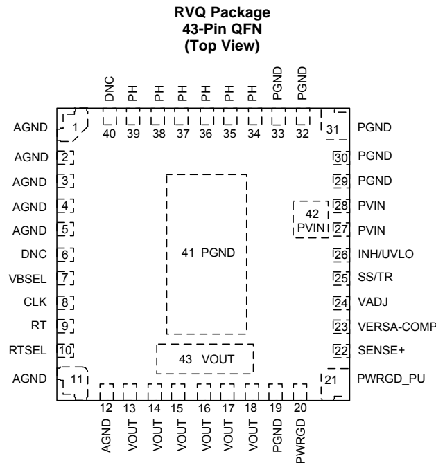
Pin Functions
