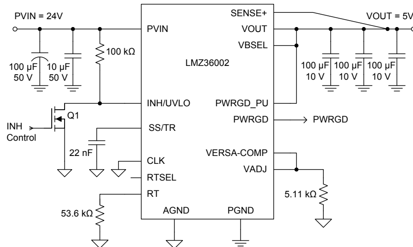
Figure 36. LMZ36002 Typical Schematic
