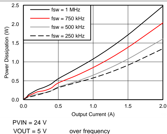
Figure 12. Power Dissipation vs Output Current over frequency
