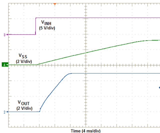
Figure 29. Inhibit Turn-On
