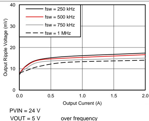
Figure 10. Voltage Ripple vs Output Current over frequency
