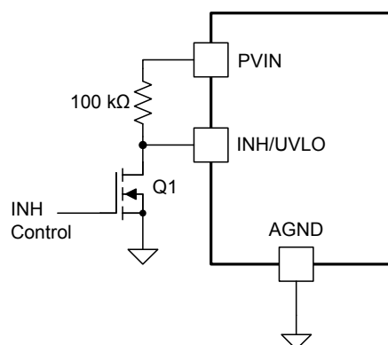
Figure 27. Typical Inhibit Control
