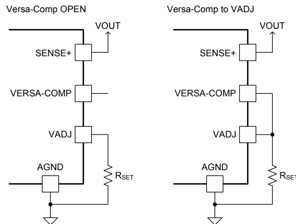
Figure 25. Versa-Comp Configurations
