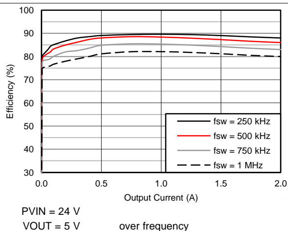
Figure 8. Efficiency vs Output Current over frequency
