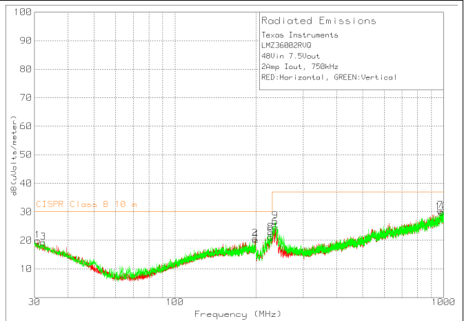
Figure 44. Radiated Emissions (EN55022 Class B) 48-V Input, 7.5-V Output, 2-A Load, 750 kHz
