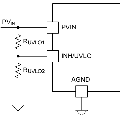
Figure 30. Adjustable PVIN UVLO
