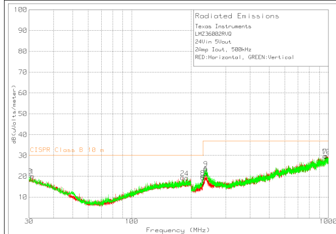
Figure 43. Radiated Emissions (EN55022 Class B) 24-V Input, 5-V Output, 2-A Load, 500 kHz
