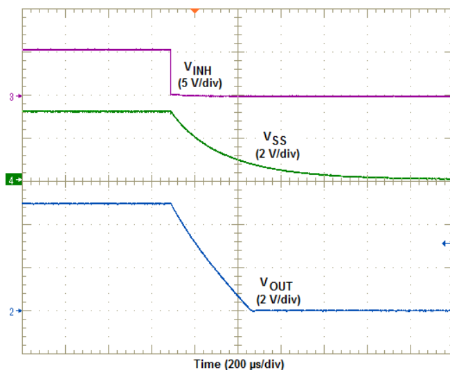
Figure 28. Inhibit Turn-Off
