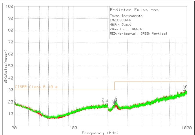
Figure 42. Radiated Emissions (EN55022 Class B) 48-V Input, 5-V Output, 2-A Load, 300 kHz
