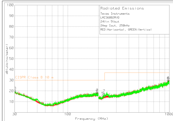
Figure 41. Radiated Emissions (EN55022 Class B) 24-V Input, 5-V Output, 2-A Load, 250 kHz
