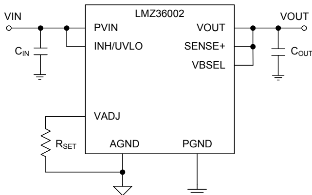
Simplified Schematic
