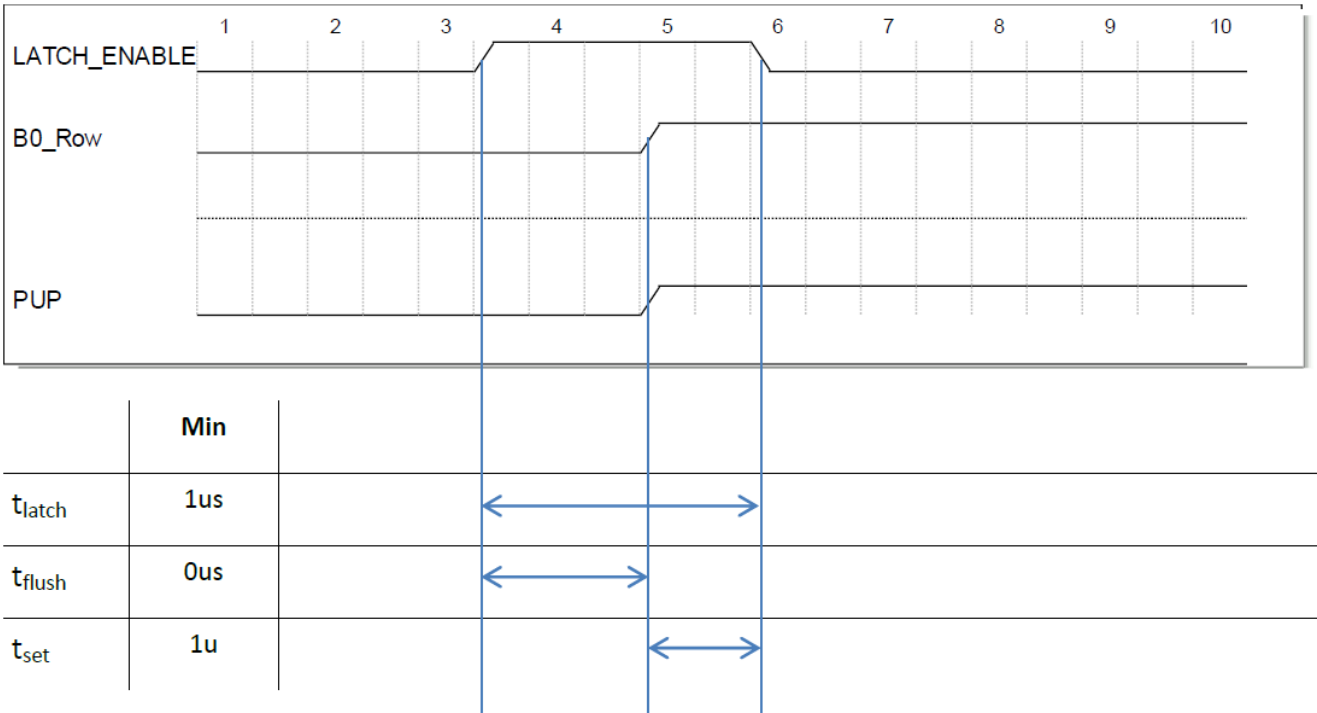
Figure 7: Device control
