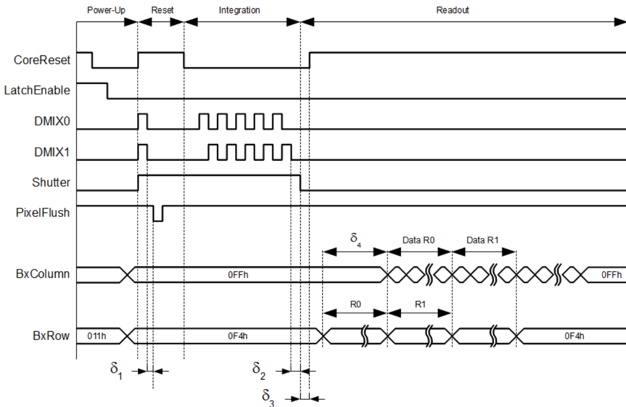
Figure 6: Global shutter timing \delta_1 \geq 0.1\mu s , \delta_2 \geq 0.1\mu s , \delta_3 \geq 1\mu s , \delta_4 \geq 1\mu s . Each cycle consists of a reset phase, an integration phase and a read-out phase.
