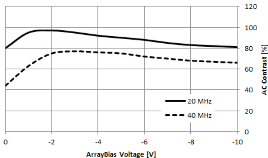
Figure 5: Typical AC demodulation contract in function of ARRAYBIAS voltage, at 20 MHz and 40 MHz demodulation frequency
