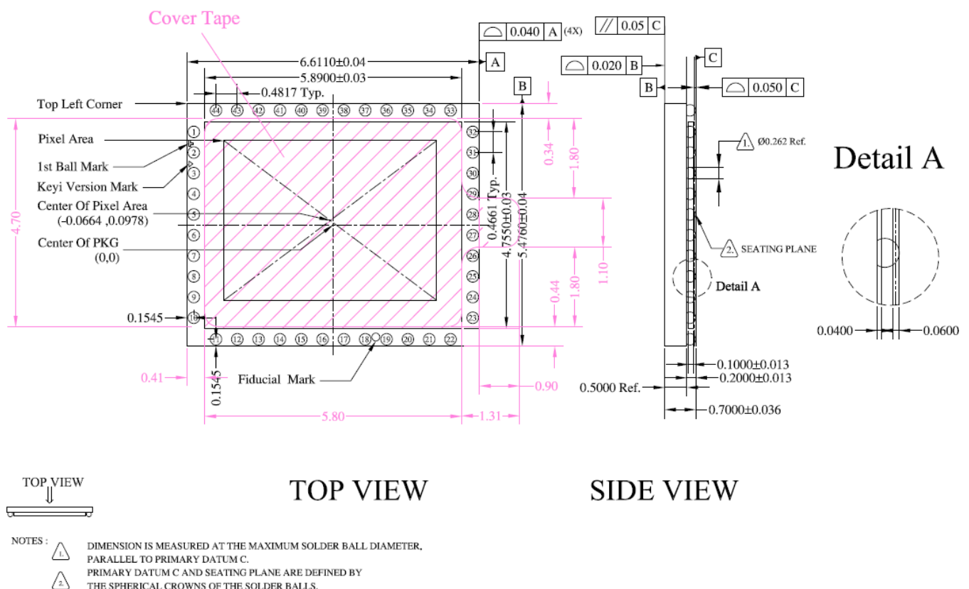
Figure 11: Mechanical & cover tape dimensions
