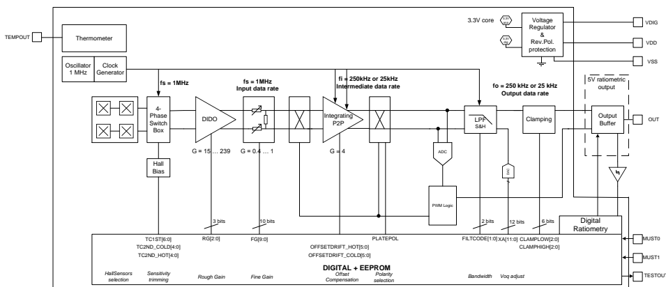
Figure 1: Block diagram
