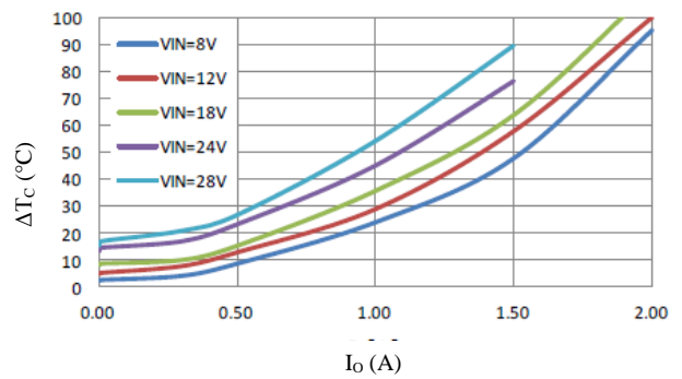
Figure 12-4 Temperature rise
