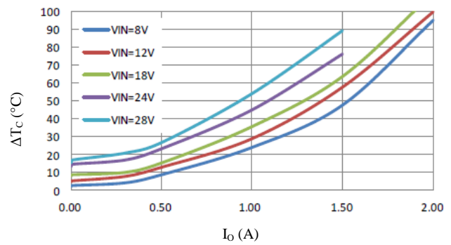
Figure 12-8 Temperature rise
