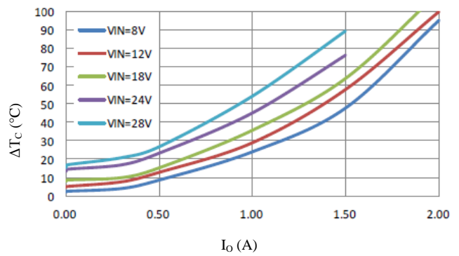
Figure 12-12 Temperature rise
