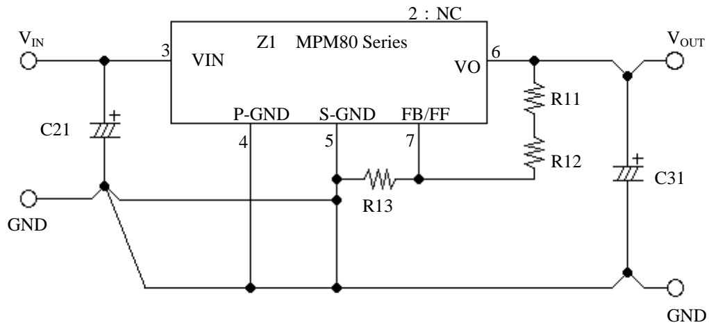
Figure11-2 Circuit diagram of pattern layout
