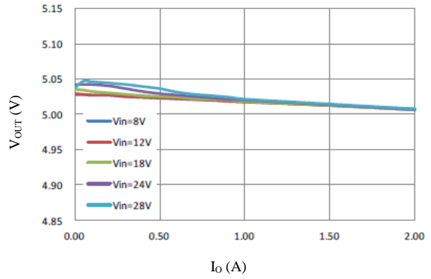
Figure 12-10 Load regulation
