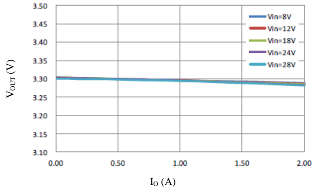
Figure 12-6 Load regulation
