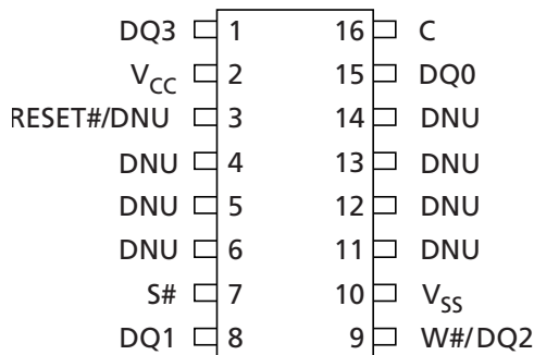
Figure 7: 16-Pin, Plastic Small Outline – SO16 (Top View)
