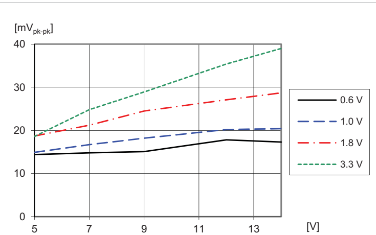
Output Ripple vs. Input Voltage
