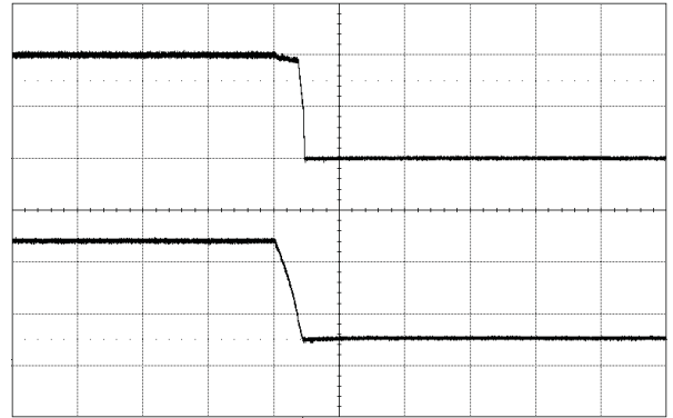
Shut-down enabled by disconnecting V_I at: T_{P1} = +25\text{ }^\circ\text{C} , V_I = 12\text{ V} , V_O = 1.0\text{ V} C_O = 470\text{ }\mu\text{F}/10\text{ m}\Omega , I_O = 50\text{ A} Top trace: output voltage (0.5 V/div.). Bottom trace: input voltage (5 V/div.). Time scale: (2 ms/div.).
