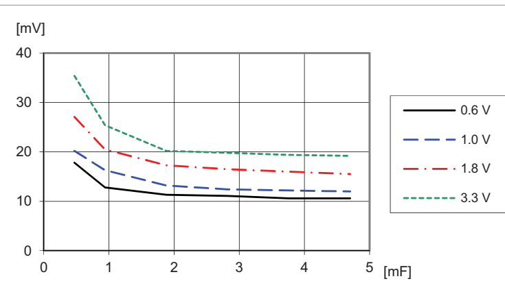
Output Ripple vs. External Capacitance
