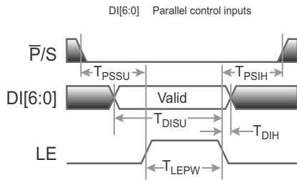
Figure 4 • Latched-Parallel/Direct-Parallel Timing Diagram
