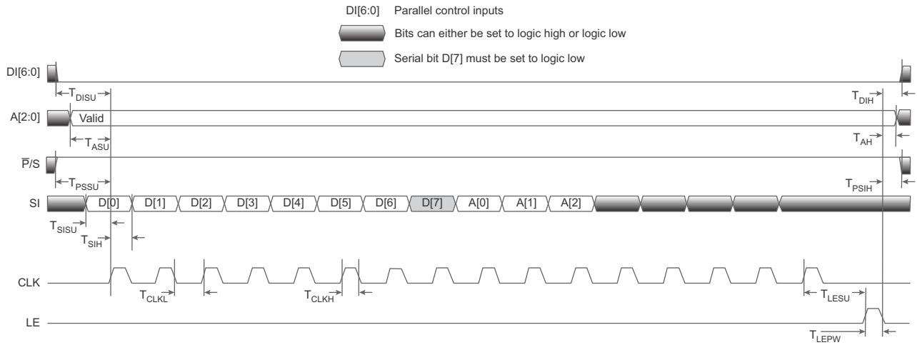
Figure 3 • Serial Addressable Timing Diagram
