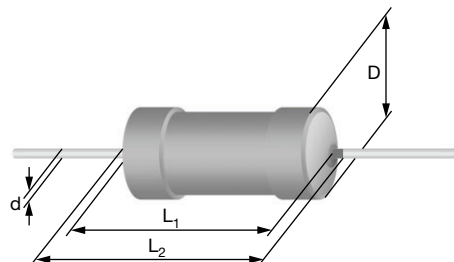
Type with straight leads
