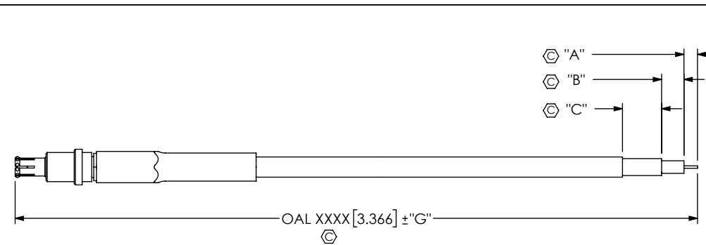
FIG 2 RF179-73SPX-172849-XXXX SHOWN (SEE NOTE 5 & 7)
