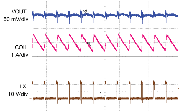
Fig. 7 - Steady-State, I_{OUT} = 3\text{ A} Time = 2\ \mu\text{s/div}
