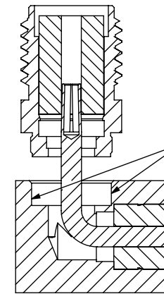
IN-PROCESS 3 ADD ADHESIVE TO BODY
