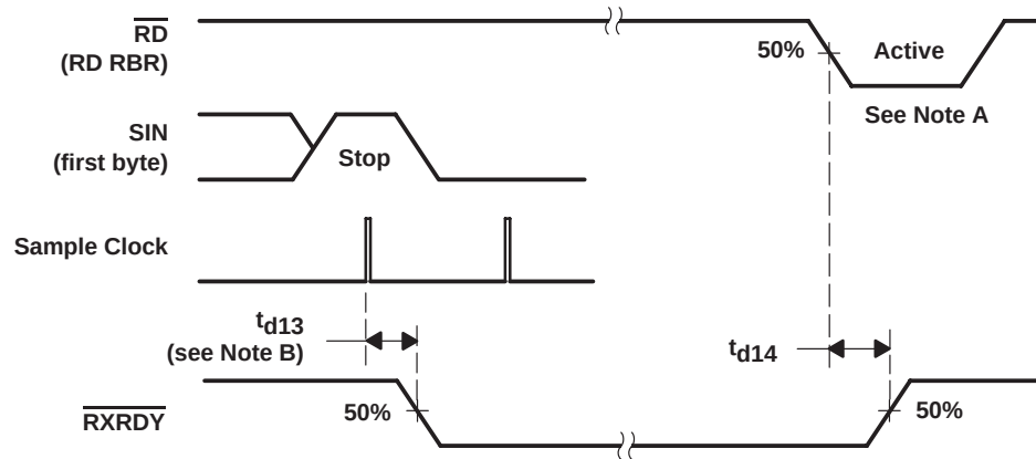
Figure 11. Receiver Ready (RXRDY) Waveforms, FCR0 = 0 or FCR0 = 1 and FCR3 = 0 (Mode 0)
